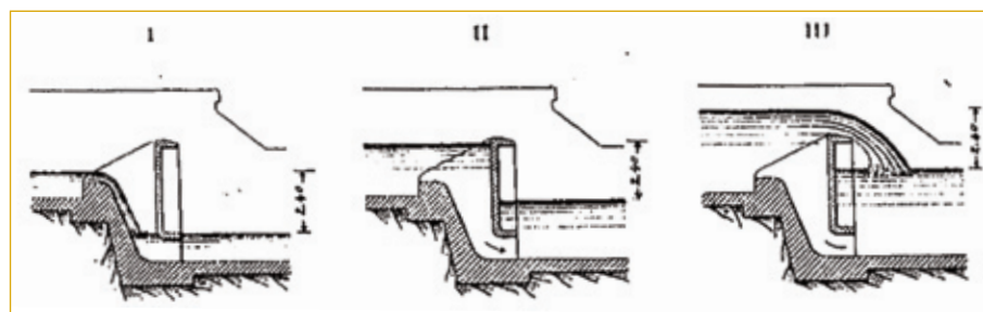
Figure 5. Functioning of the stilling basin structures. [1]
