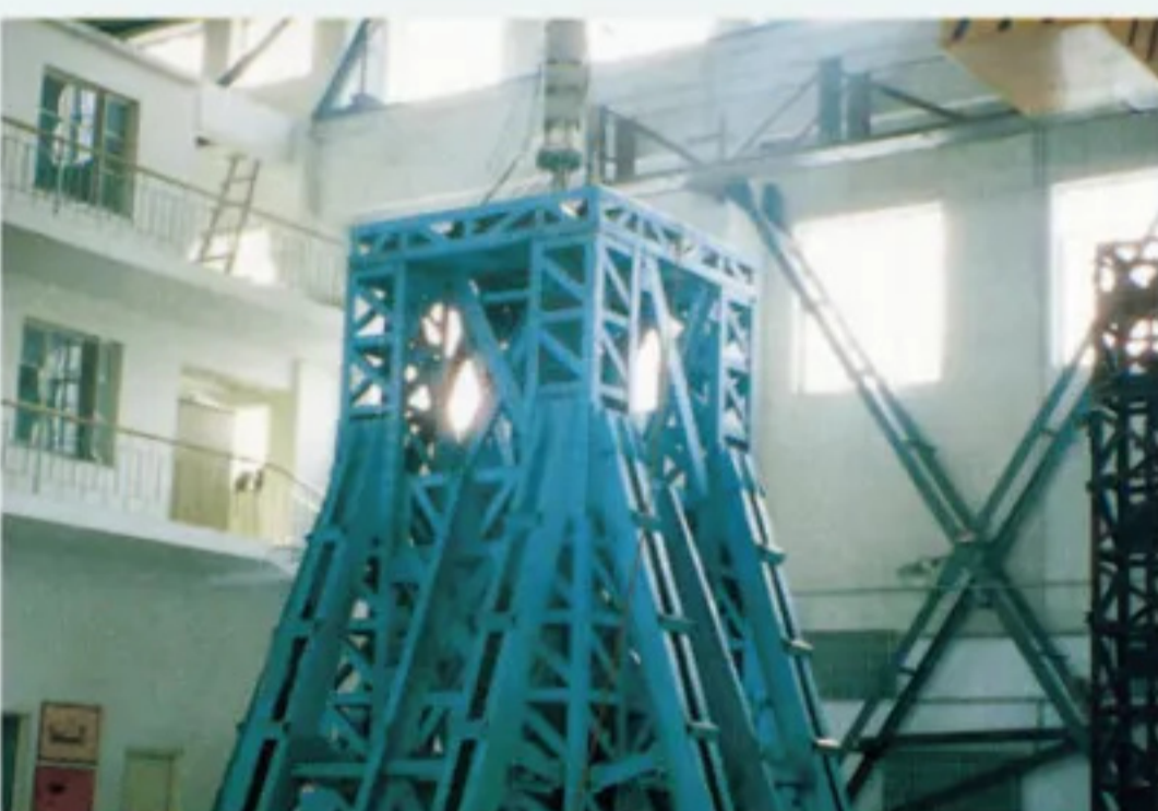
Tri-axial earthquake simulating shaking table with 6 degrees of freedom
